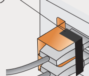
●AUK-01-01-B USB-TypeB+USB (無停電電源装置) USB TypeB+ UPS
